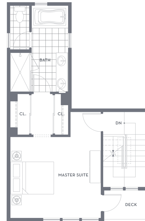
THIRD LEVEL
